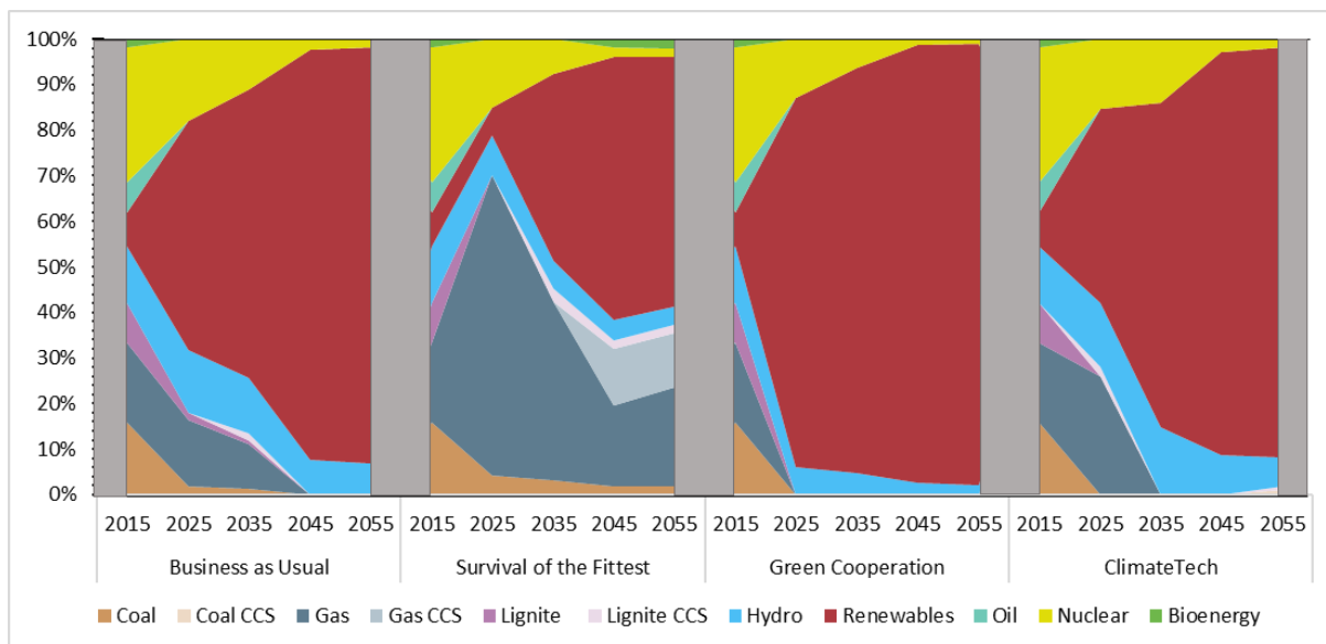
Figure 10: Electricity mix for the European Union in the four scenarios
