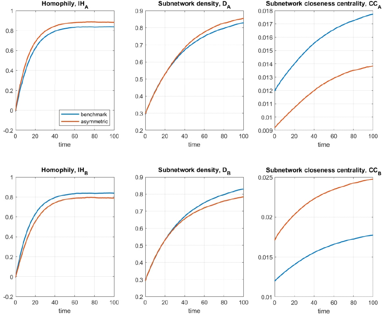
Figure 4.a Evolution of network \gamma_t varying the sizes of subgroups A and B . Benchmark calibration ( N_A = N_B = 50 ) is compared to a case of asymmetric groups with N_A = 65 and N_B = 35 .
