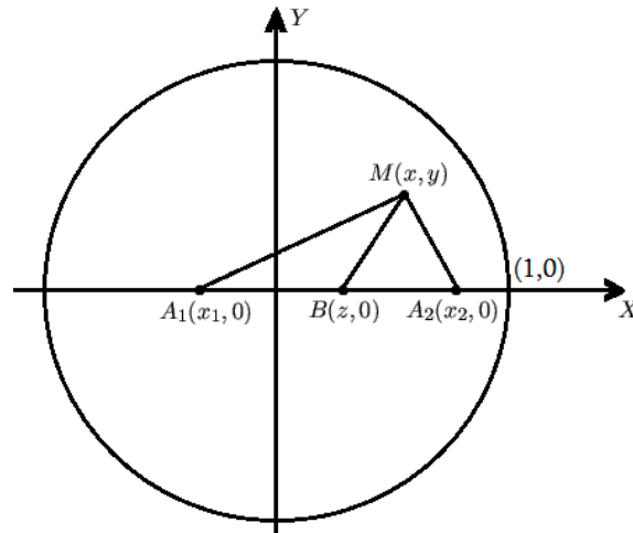
Figure 1: location on the diameter of the disk
