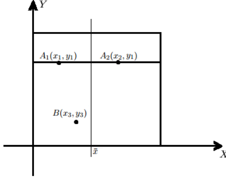
Figure 3: Location Game on a Square
