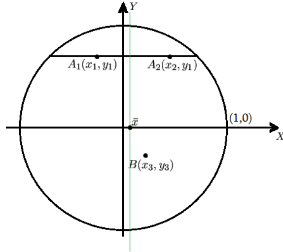
Figure 2: introducing the street
