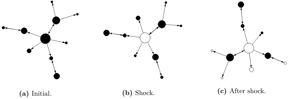
Figure 4.1: The contagion process after the default of the largest component (B1) and its shock to the network where \rho = 1\% of L and \frac{b_{interbank}^s}{b^s} = 0.5 for all components of the scale-free network (The black nodes are solvent banks and the white ones are insolvent banks in each level).
