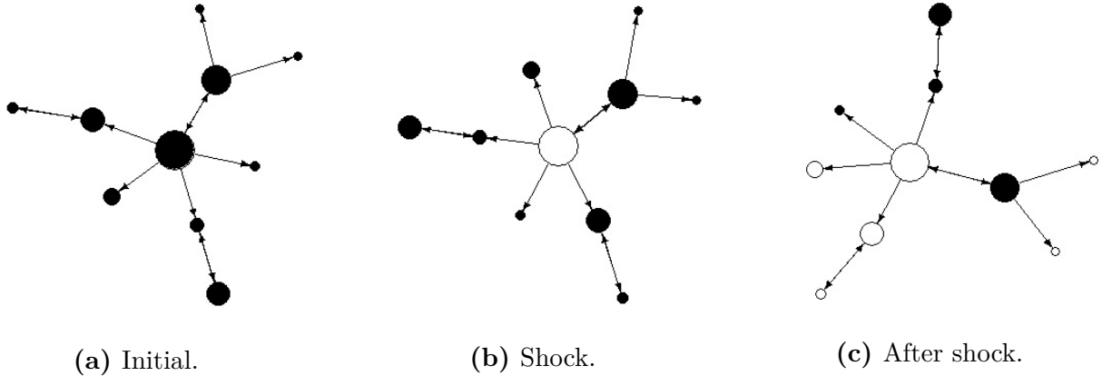
Figure 4.2: The contagion process after the default of the largest component (B1) and its shock to the network where \rho = 1\% of L and \frac{b_{interbank}^s}{b^s} = 1 for all components of the scale-free network (The black nodes are solvent banks and the white ones are insolvent banks in each level).
