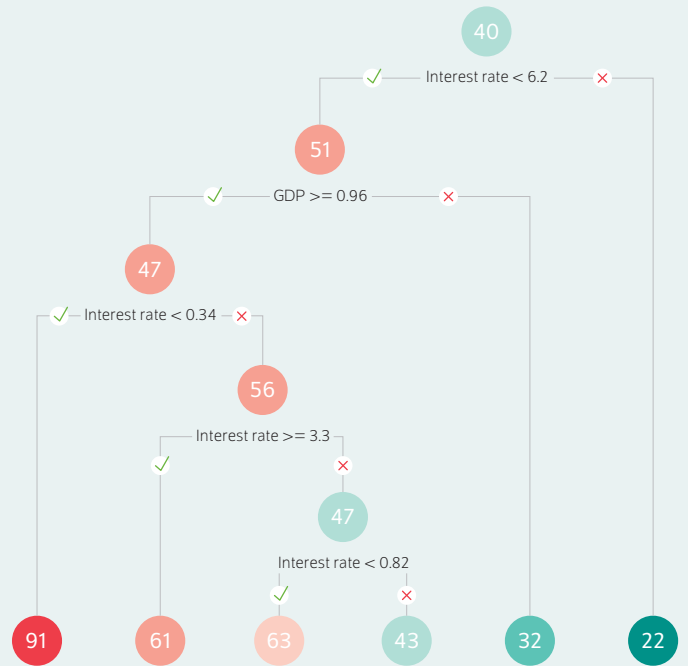
Bubble probabilities in percent for a stylized decision tree
