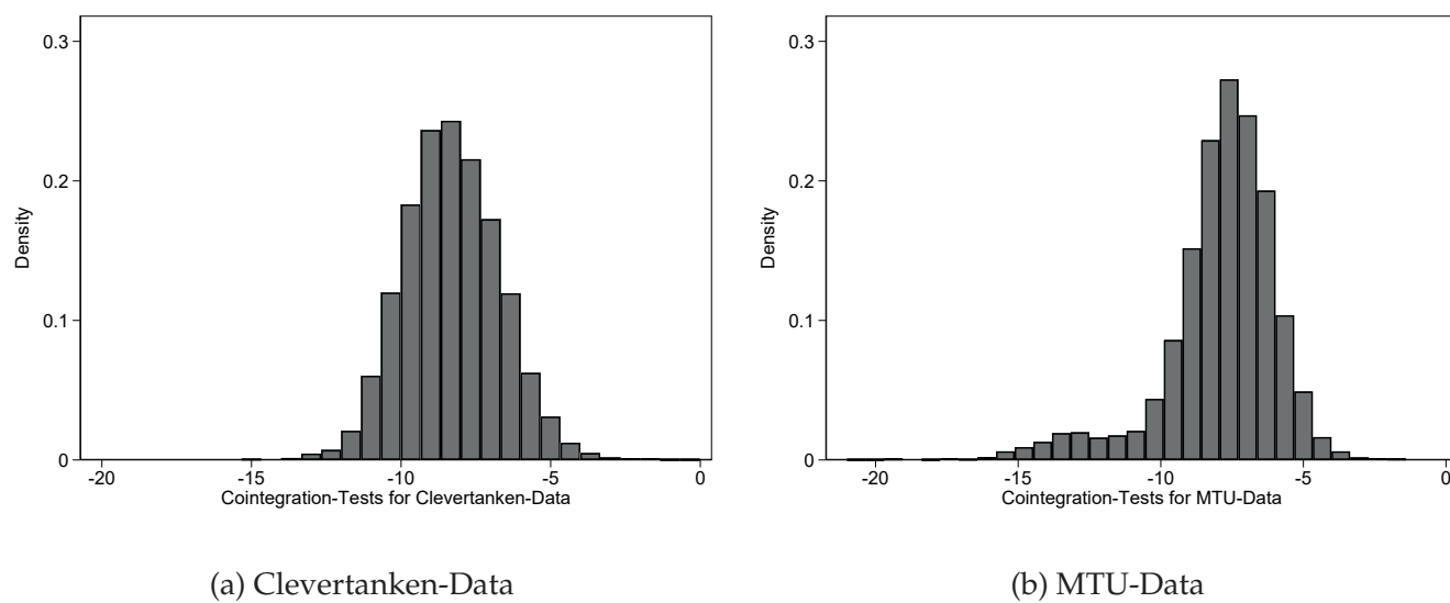
Figure A1: Cointegration-Tests for Clevertanken and MTU-Data
