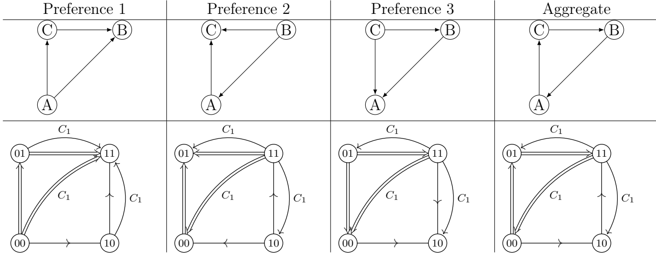
Figure 6: Combining the graphs from Example 2.1 (above) and Example 2.2 (below). Contrast the edges between A, B, C in the top graphs and the double-angled edges between 00, 11, 01 in the bottom graphs. To make the graph more readable, we omitted all labels except those of compound propositions.
