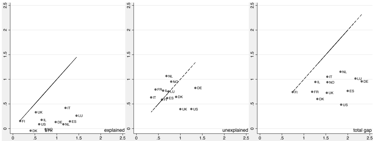
Figure 6: Explained, unexplained and total gender earnings gaps for birth cohorts 1935 (x-axis) vs. cohort 1980 (y-axis) – linear predictions
