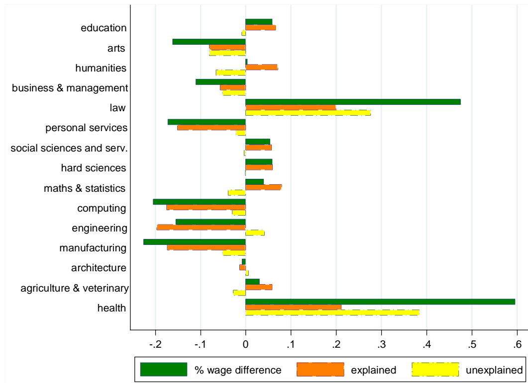
Figure 2: Oaxaca-Blinder Decomposition
