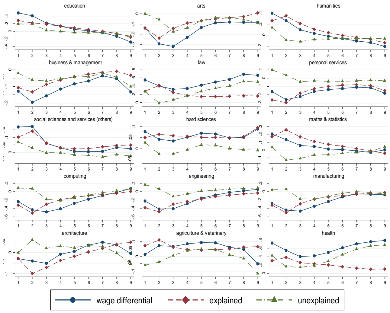
Figure 4: RIF-Regression Decomposition
