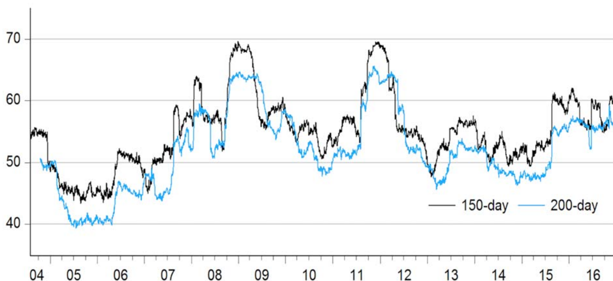
Figure 5: Dynamic Total Volatility Connectedness – 63 SEACEN Region Banks (January 5, 2004 - December 31, 2016)
