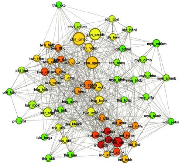
(a) June 23, 2016 (index=56%)
