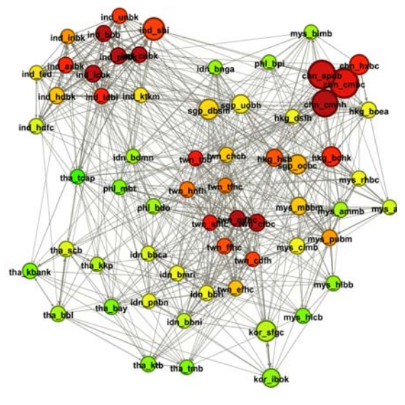
(b) Sep. 11, 2015 (index=61.3%)
