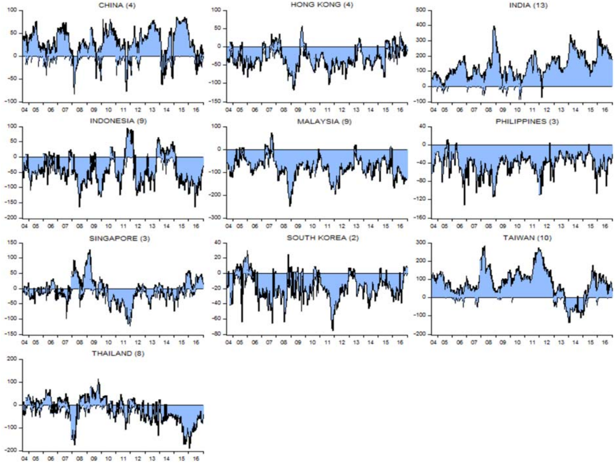
Figure 8: Country-level Dynamic Net Volatility Connectedness
