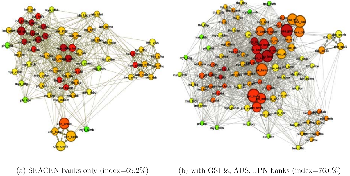
Figure 14: Global Financial Crisis – Jan. 12, 2009 (with and without GSIBs)
