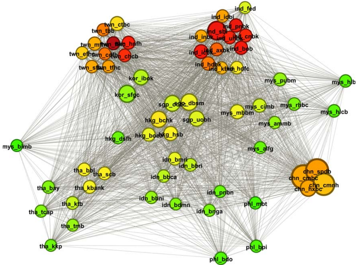
Figure 2: SEACEN Region Bank Volatility Connectedness – 63 banks. (index=48.5%) Based on pairwise directional volatility connectedness over the full-sample, from Jan 5, 2004 to December 31, 2016.
