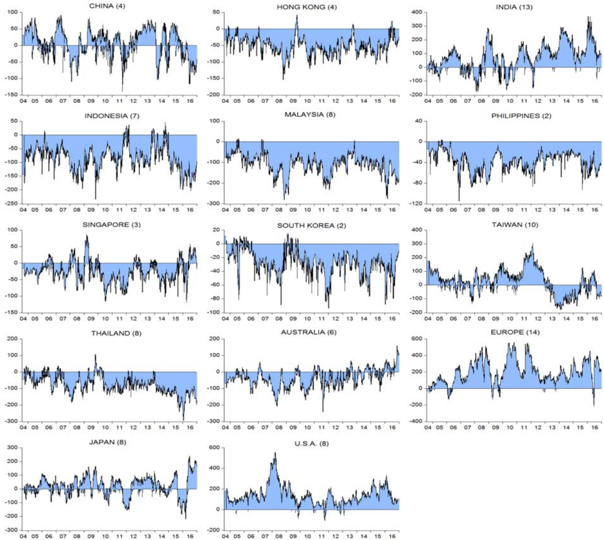
Figure 9: Country-level Dynamic Net Connectedness (with GSIBs, Australian & Japanese Banks)
