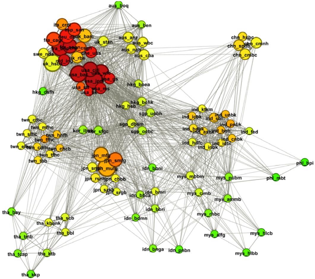
Figure 4: SEACEN Bank Volatility Connectedness, incl GSIBs, Australian and Japanese Banks (DYCI=60.1%) Based on pairwise directional volatility connectedness of 97 banks over the full-sample, from Jan 5, 2004 to December 31, 2016.
