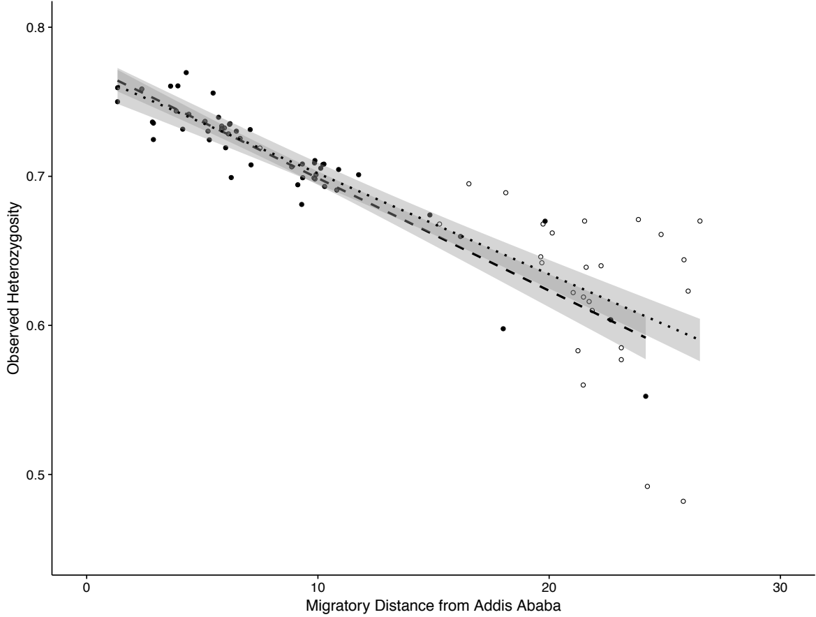
Figure 3: Observed Heterozygosity vs. Migratory Distance: Original and Wang et al. (2007) Additions
