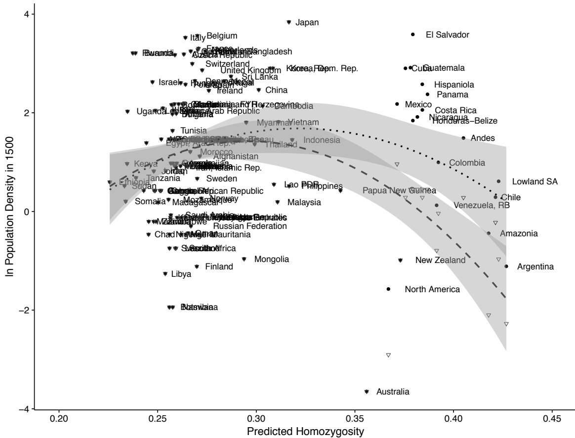
Figure 11: Density vs. Homozygosity with Updated Population Estimates (Quadratic)
