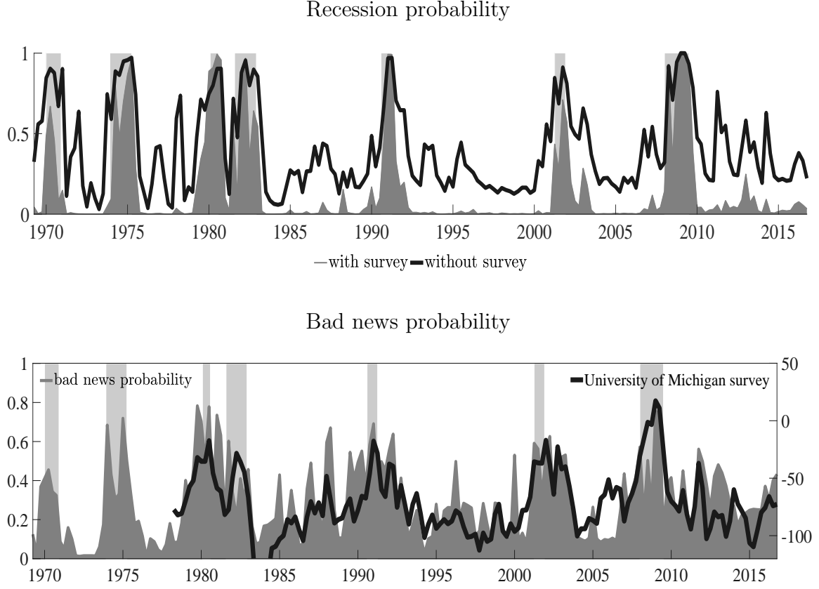
Figure 5: Filtered estimates of recession and bad news probabilities
