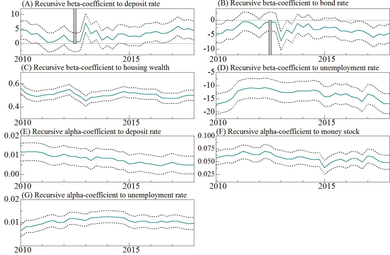
Figure 4: Rolling-window estimation based on the concentrated model for 22-year samples: (1988:3-2010:1)-(1996:3-2018:1). The dashed lines indicate the 95% confidence bands. The grey bars captures the time period in which negative monetary policy rates were introduced.
