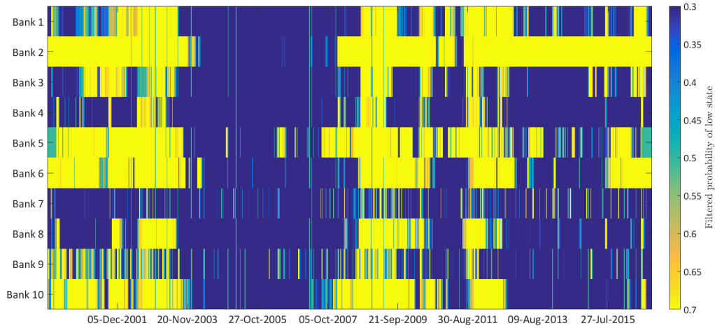
Figure B.1: Heat map for the filtered probabilities
