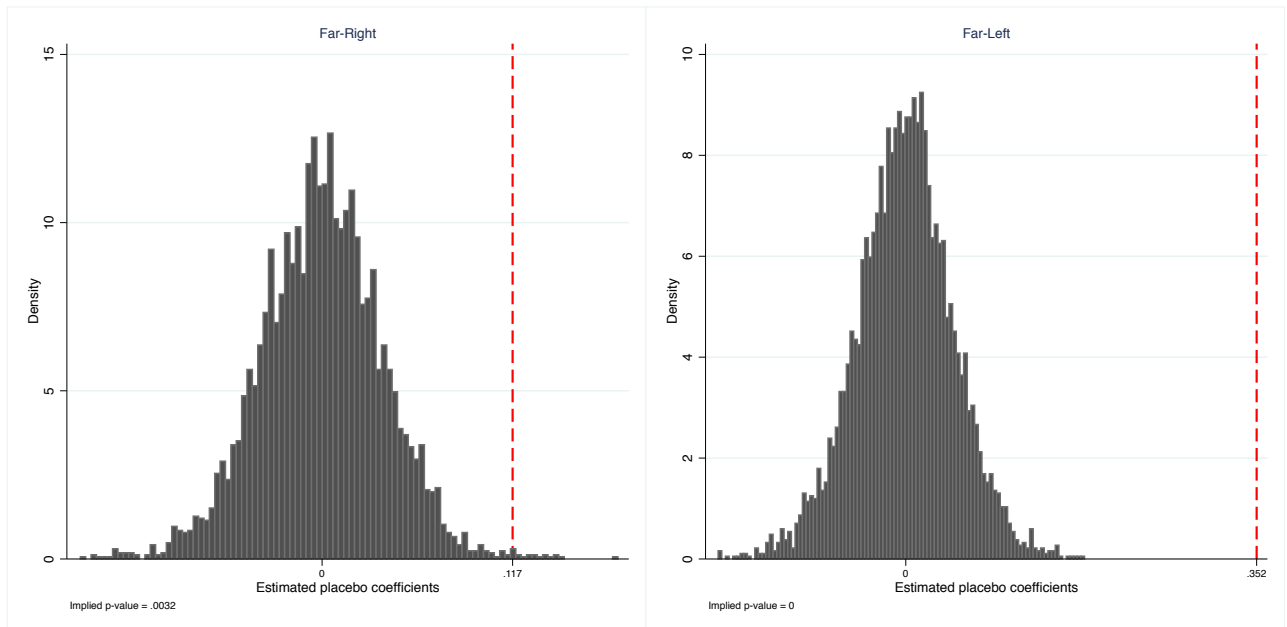
Figure 8: Permutation Tests
