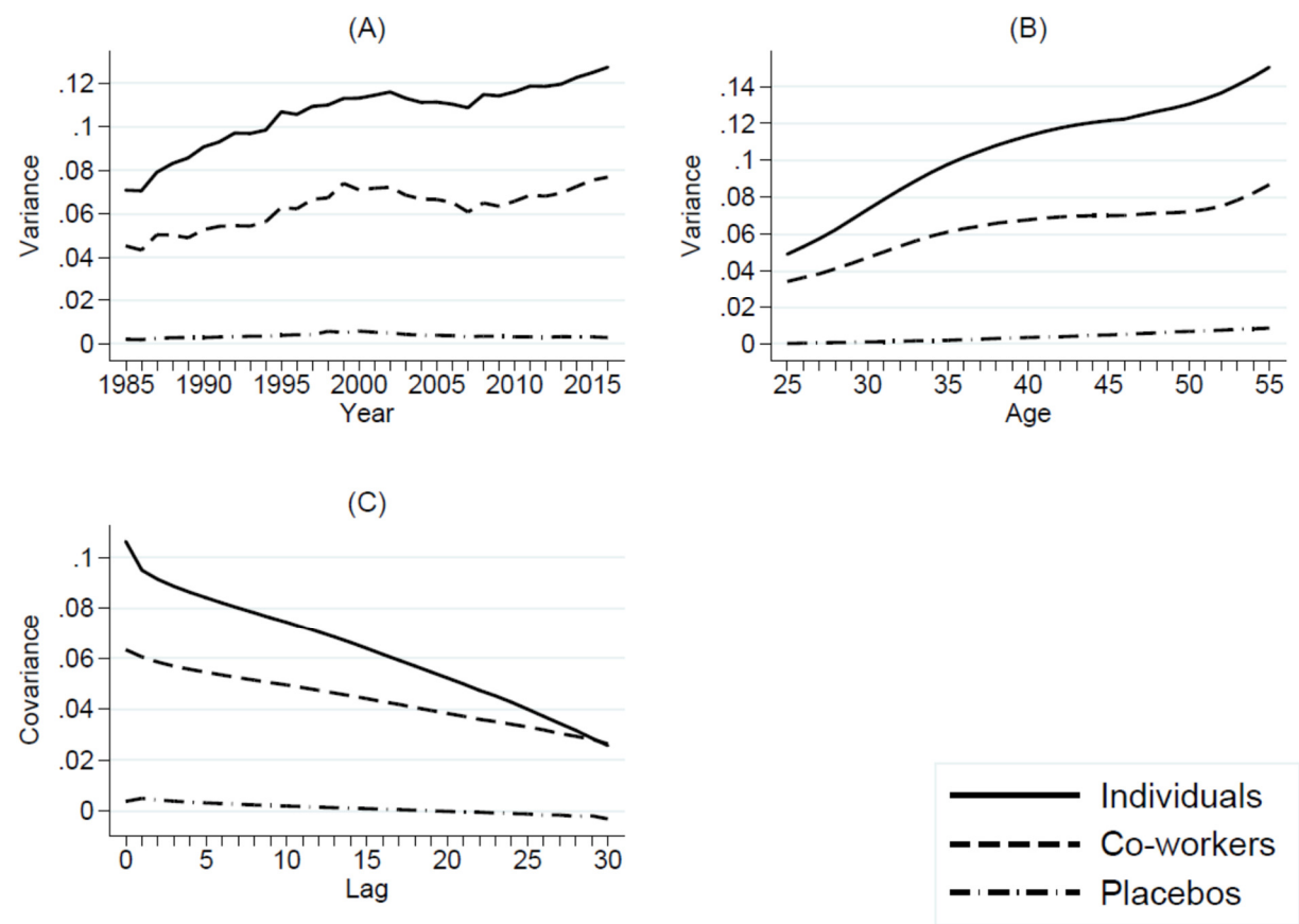
Figure 2: Empirical moments
