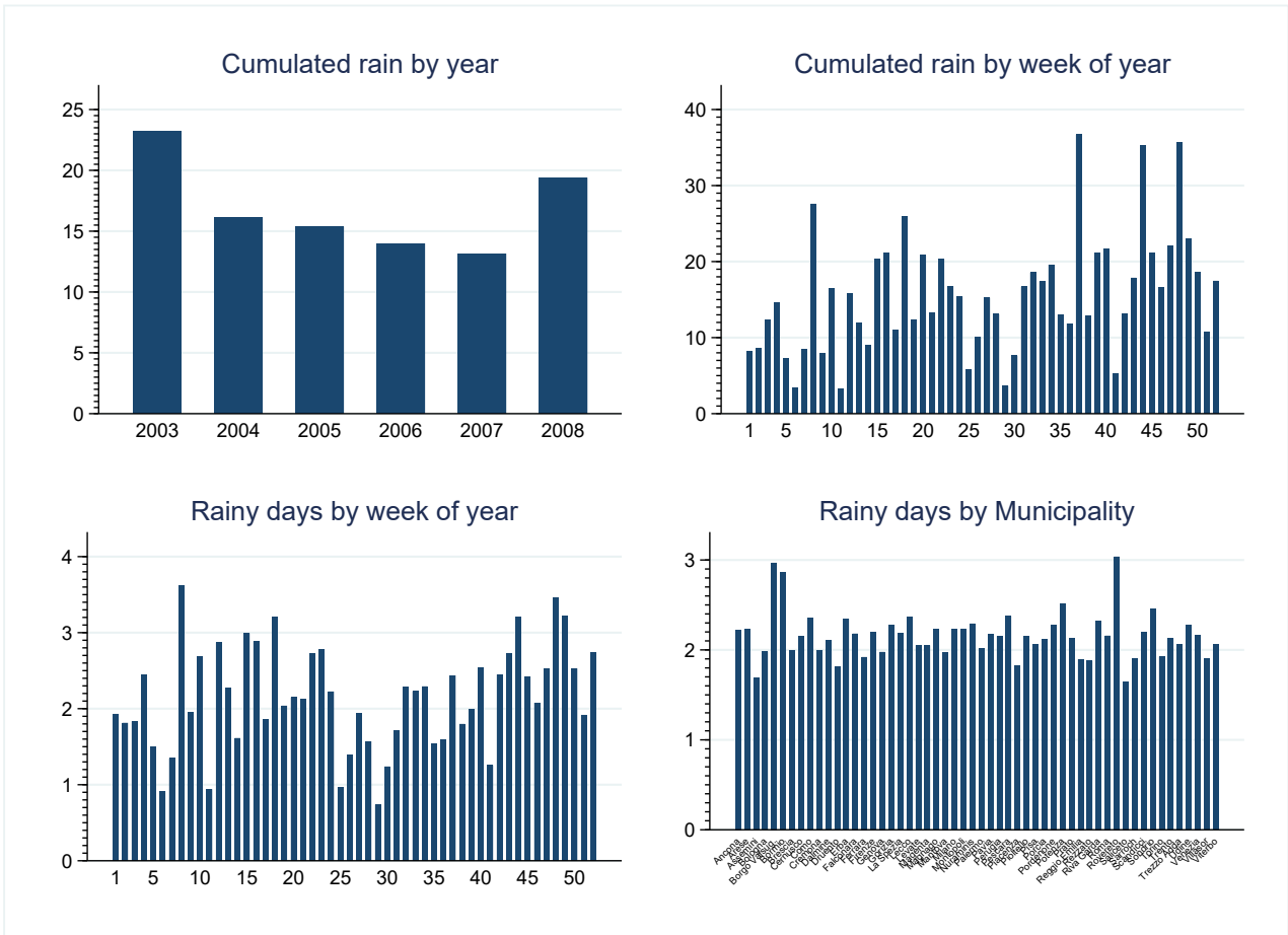
Figure 3: Rain Distribution
