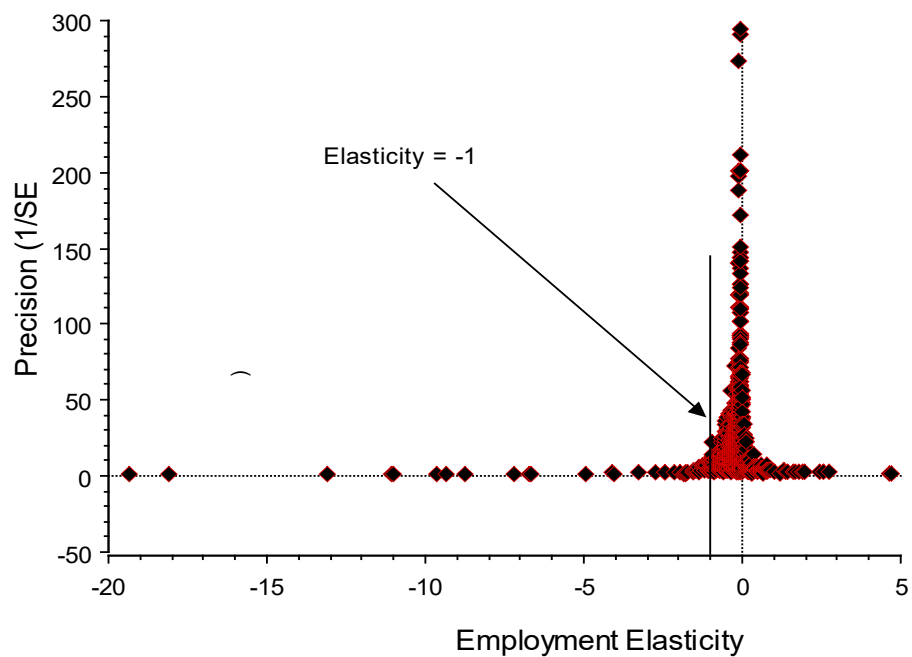
Figure A3. Funnel Plot of US Minimum Wage Employment Elasticities (m=1,474)
