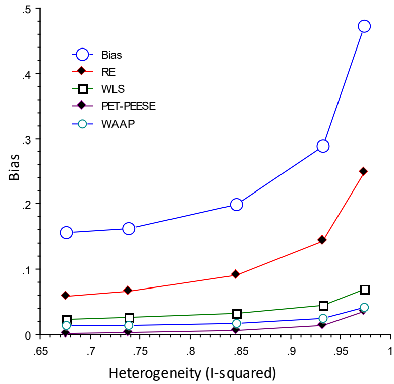
Figure A4: Biases (proportional heterogeneity, \eta=0 , and m=400 )
