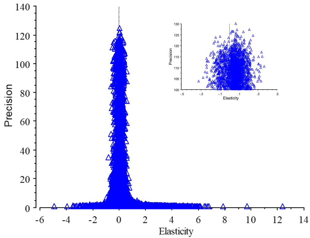
Figure A1. Funnel Graph of Simulated Elasticities and their Precisions ( \eta = 0 , 50% Publication Selection, I^2=94\% , 100,000 replications)
