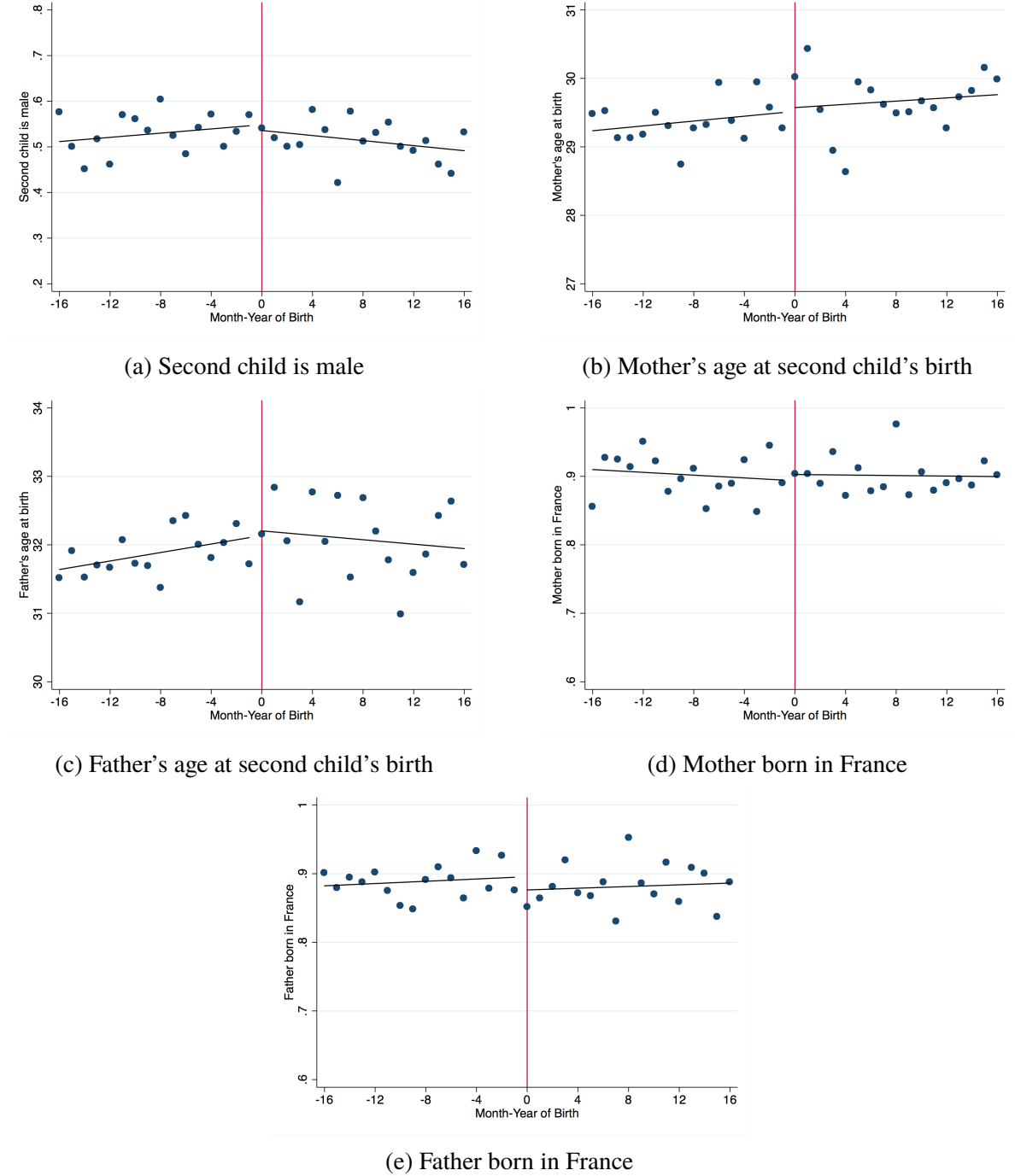
Figure A1: Smoothness of baseline covariates
