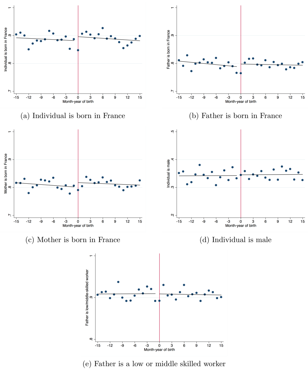
Figure 3: Covariate balance
