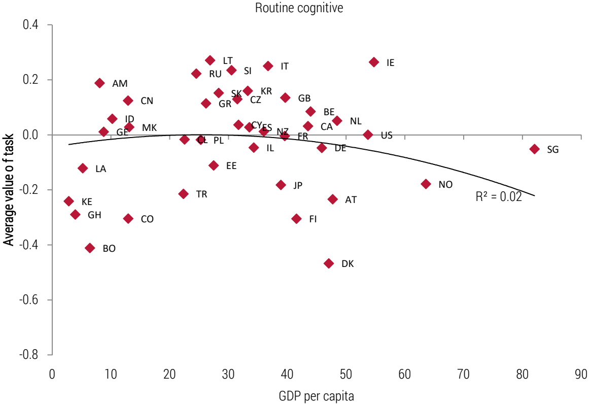
Figure 3 (cont'd). The average values of tasks against GDP per capita.
