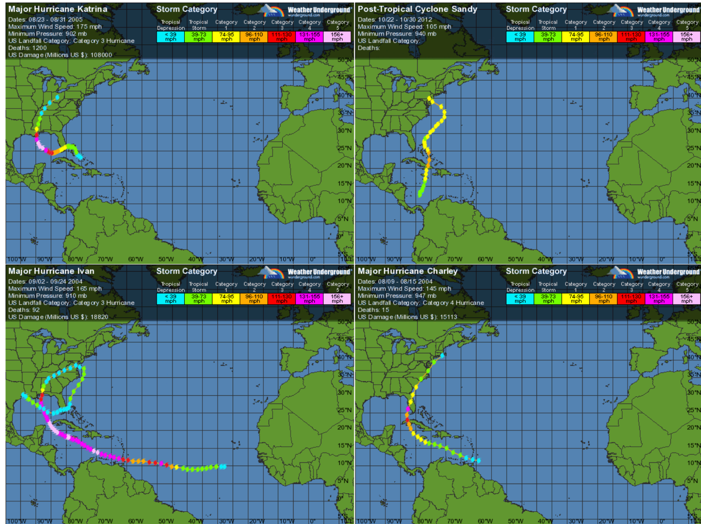
Figure 2: Hurricane trajectories
