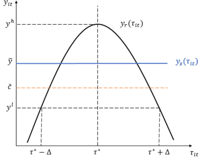
Figure 1: Crop yield as a function of temperature
