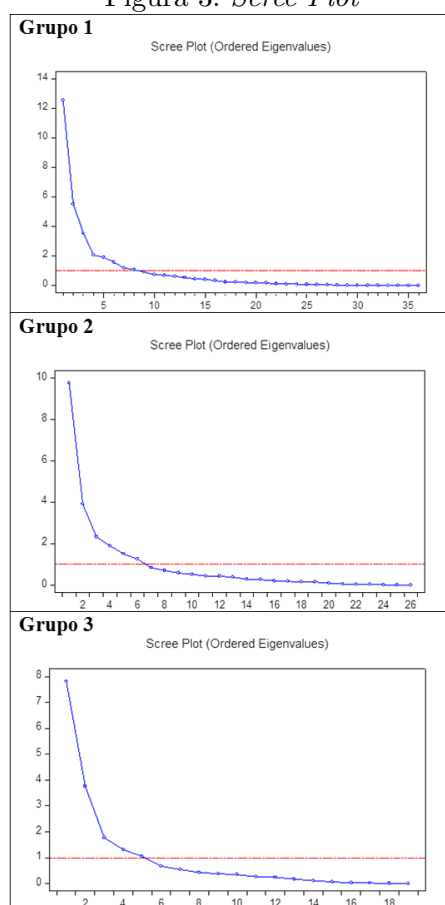
Figura 3: Scree Plot
