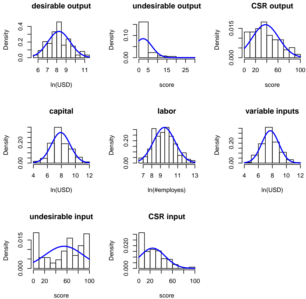
Figure 1: Histogram of the variables used in the empirical analysis
