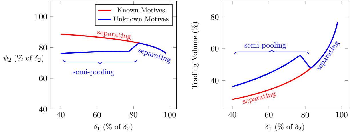
Figure 3: Equilibrium as a Function of Low Type's Quality ( \delta_1 )
