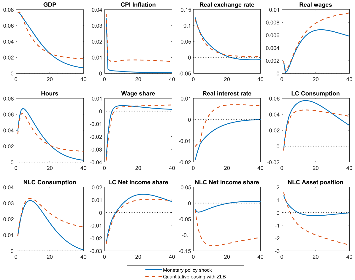
Figure 1: Impulse responses for expansionary short-term rate and QE shock
