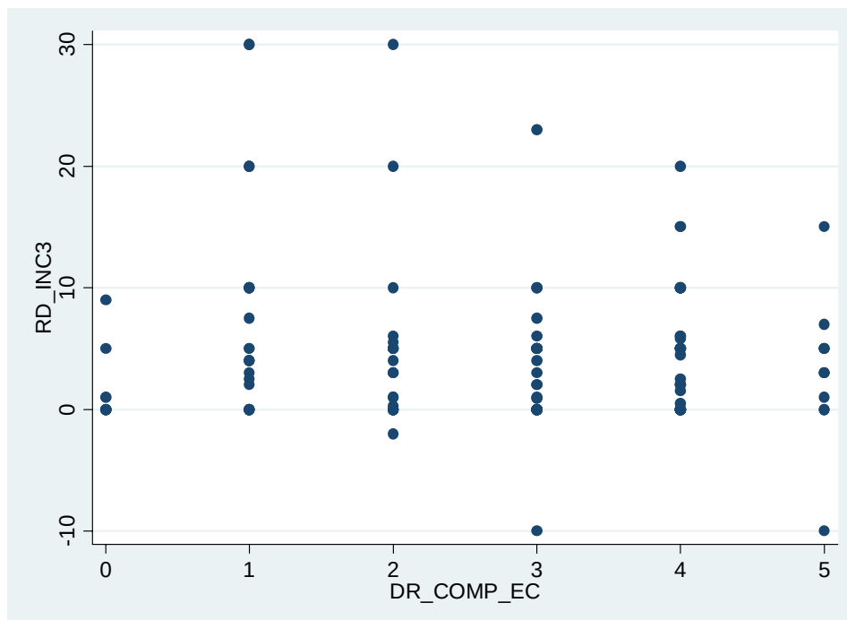
Figure A2. Scatterplot between the changes in firms' R&D investment in the three years to come (RD_INC3) and the importance of competition from companies located in emerging countries, e.g. China or India (DR_COMP_EC)
