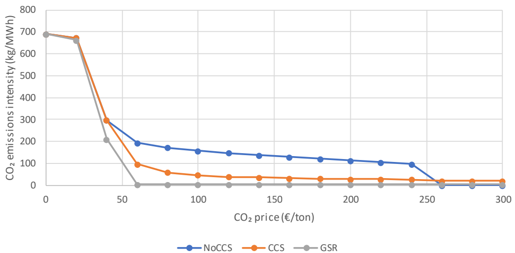
Figure 4: Marginal CO 2 abatement cost curves for the three scenarios.
