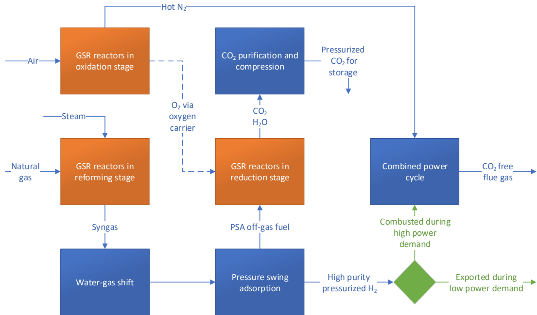
Figure 1: Simplified flow diagram of the GSR plant for flexible power or hydrogen production. The green diamond represents the switch between power and hydrogen operating modes.
