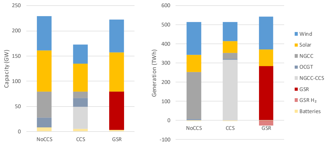
Figure 2: Capacity and annual generation for the optimal technology mix in the three scenarios.
