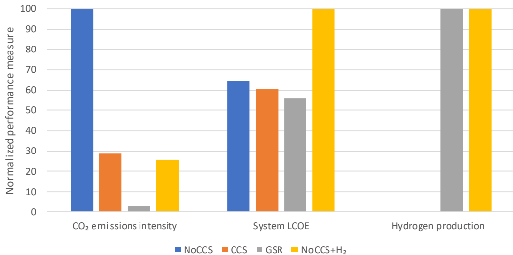
Figure 3: Normalized comparison of the four scenarios in terms of three key performance metrics. Here, a value of 100 represents a CO 2 emissions intensity of 157 kg/MWh, a system levelized cost of electricity (LCOE) of 121 €/MWh, and hydrogen production of 453 TWh/year. System LCOE is quantified as the total system cost (Equation 10) divided by the total annual electricity demand.
