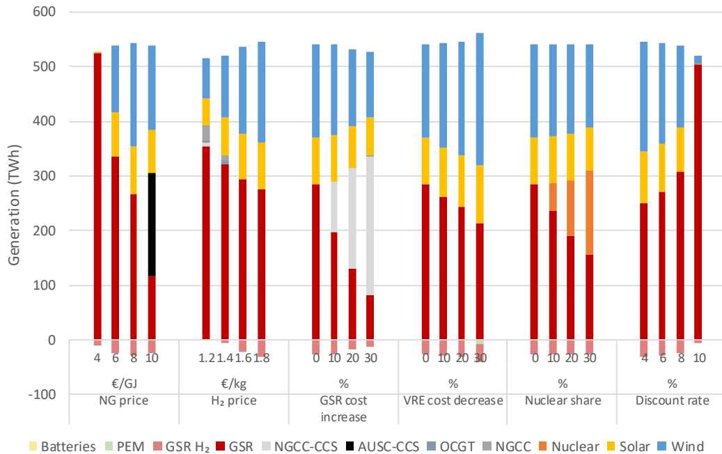
Figure 6: Sensitivity of the GSR scenario to changes in six important model parameters.
