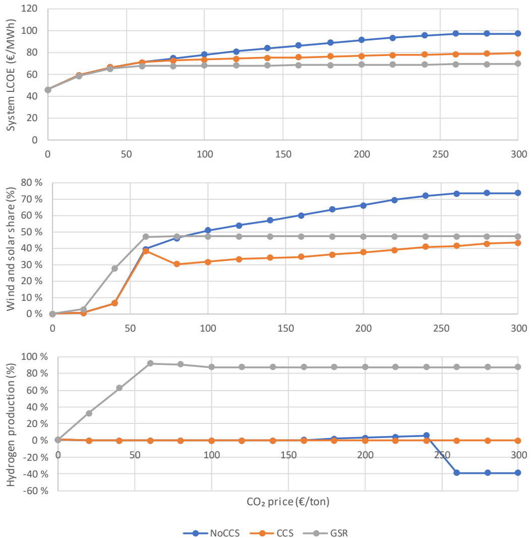
Figure 5: More details of scenario performance across different CO 2 prices. Hydrogen production is expressed as a fraction of total annual electricity demand.
