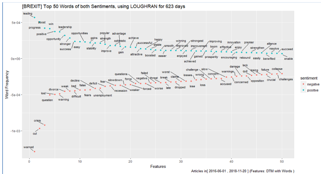
Fig. 3. Distribution of top 50 positive and negative words according to LOUGHRAN
