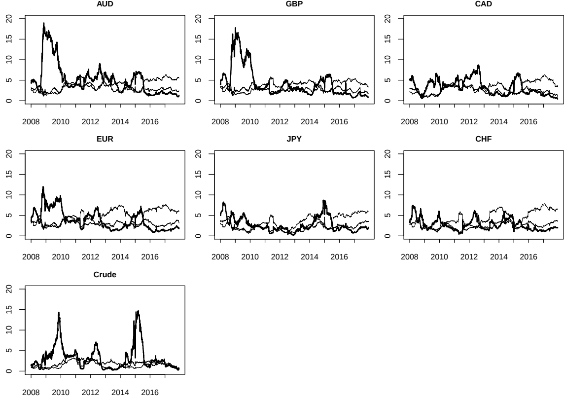
Figure 5: Directional (TO) frequency connectedness. The frequency connectedness at short-term horizon defined at d_1 \in [1, 5] days in solid line, medium-term horizon defined at d_2 \in (5, 20] days medium bold line, and long-term horizon defined at d_3 \in (20, 300] days in bold line. Note that all lines through the frequency bands d_s sum to the total connectedness. The directional (TO) frequency connectedness quantifies how volatility (measured at given frequency) from a specific asset (oil or currency) transmits to other assets in portfolio (“contribution TO”).
