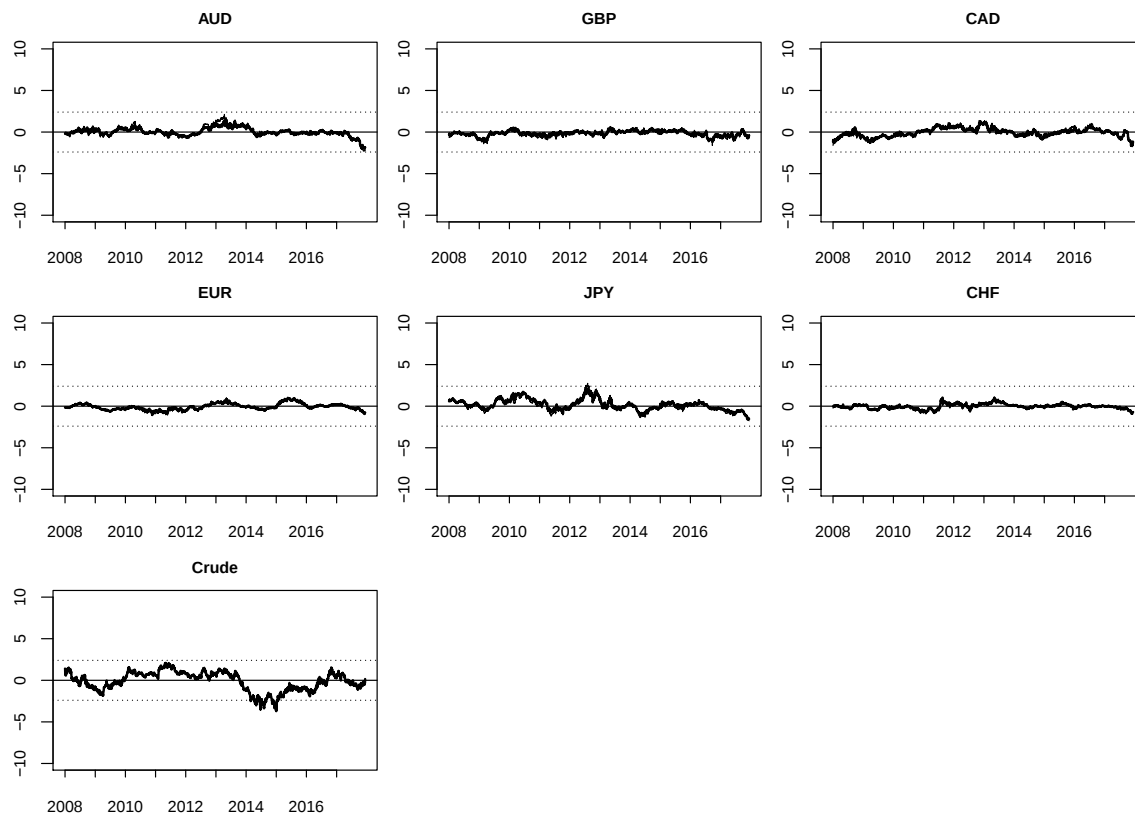
Figure 4: Directional (FROM) Spillover asymmetry measure (SAM). Solid line represents the directional SAM for the forex market only, while the bold solid line represents the directional SAM for the crude oil and forex markets. 95% bootstrapped confidence bands are shown by dotted lines. The directional SAM (FROM) quantifies how asymmetry in volatility from a group of assets transmits to a specific asset (oil or currency) (“contribution FROM”).
