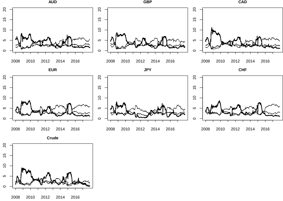
Figure 6: Directional (FROM) frequency connectedness. The frequency connectedness at short-term horizon defined at d_1 \in [1, 5] days in solid line, medium-term horizon defined at d_2 \in (5, 20] days medium bold line, and long-term horizon defined at d_3 \in (20, 300] days in bold line. Note that all lines through the frequency bands d_s sum to the total connectedness. The directional (FROM) frequency connectedness quantifies how volatility (measured at given frequency) from a group of assets transmits to a specific asset (oil or currency) (“contribution FROM”).
