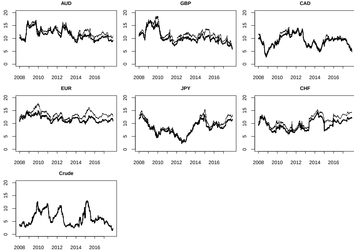
Figure 1: The directional (TO) volatility connectedness of six currencies (solid line), the directional volatility connectedness of six currencies and crude oil (bold solid line). The directional (TO) volatility connectedness quantifies how volatility from a specific asset (oil or currency) transmits to other assets in portfolio (“contribution TO”).
