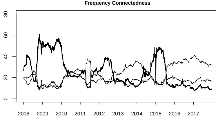
Figure 4: Dynamic frequency connectedness. The frequency connectedness at the short-term horizon defined at d_1 \in [1, 5] days is marked with the solid line, the medium-term horizon defined at d_2 \in (5, 20] days is depicted by the medium bold line, and the long-term horizon defined at d_3 \in (20, 300] days is represented with the bold line. Note that all lines through the frequency bands d_s sum to the total connectedness.
