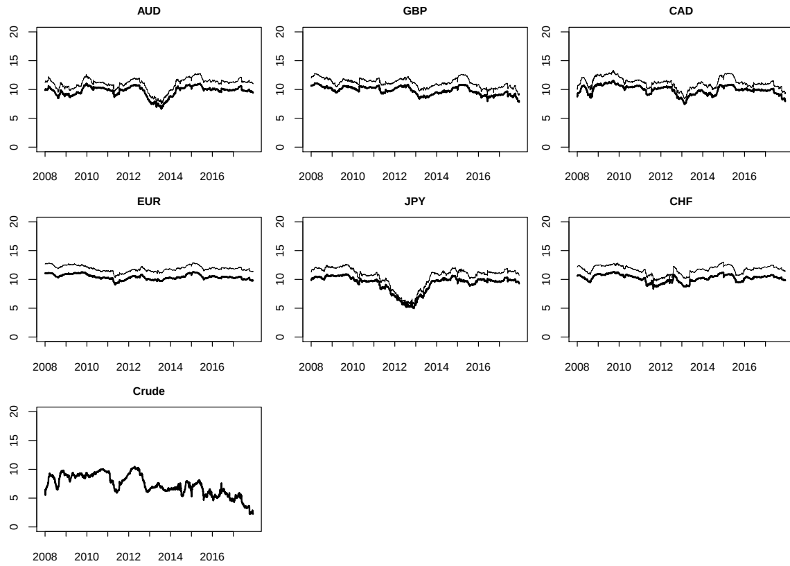
Figure 2: The directional (FROM) volatility connectedness of six currencies (solid line), the directional volatility connectedness of six currencies and crude oil (bold solid line). The directional (FROM) volatility connectedness quantifies how volatility from a group of assets transmits to a specific asset (oil or currency) (“contribution FROM”).
