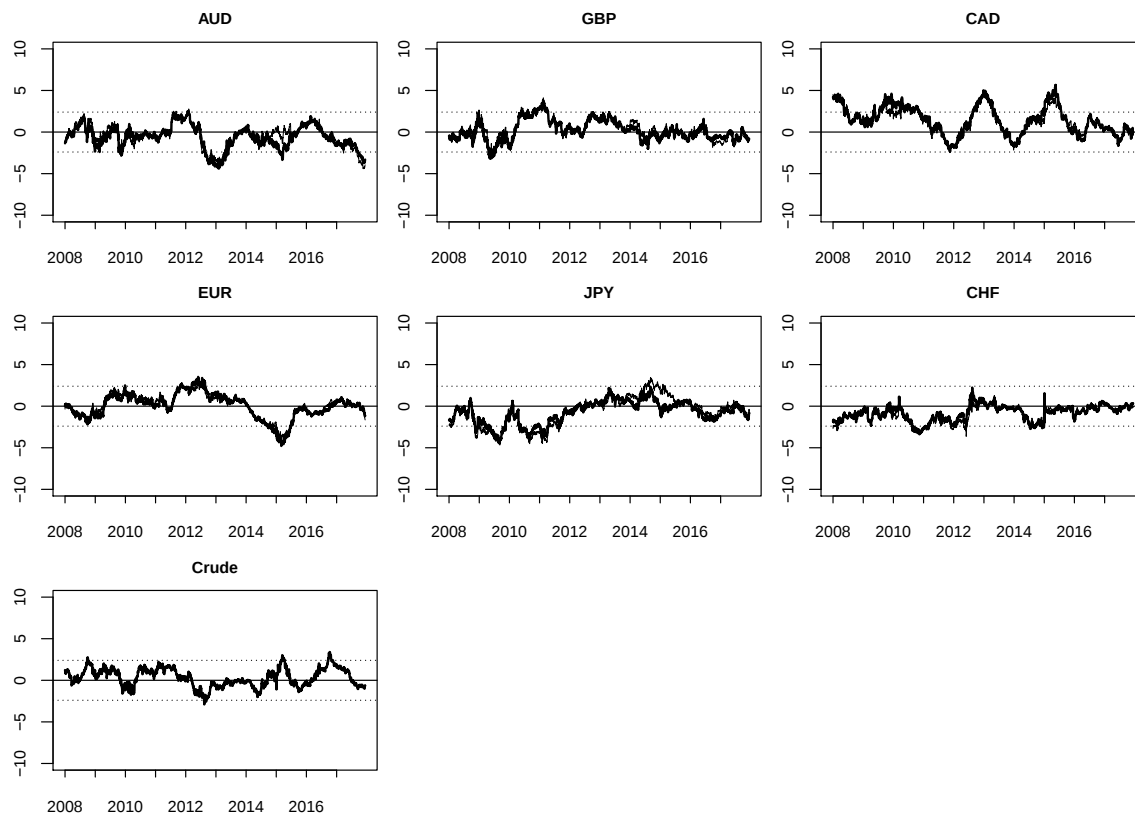
Figure 3: Directional (TO) Spillover asymmetry measure (SAM). Solid line represents the directional SAM for the forex market only, while the bold solid line represents the directional SAM for the crude oil and forex markets. 95% bootstrapped confidence bands are shown by dotted lines. The directional SAM (TO) quantifies how asymmetry in volatility from a specific asset (oil or currency) transmits to other assets in portfolio (“contribution TO”
