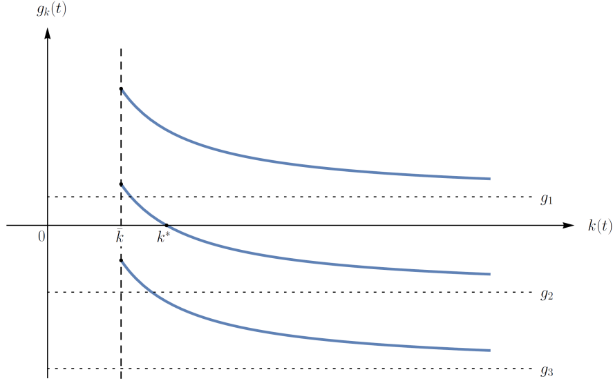
Figure 4.1: The Dynamical System of the Equilibrium.
