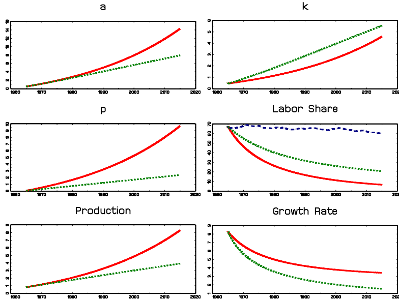
Figure 5.1: Transitional Dynamics with and without the No-arbitrage Condition (2.3)
