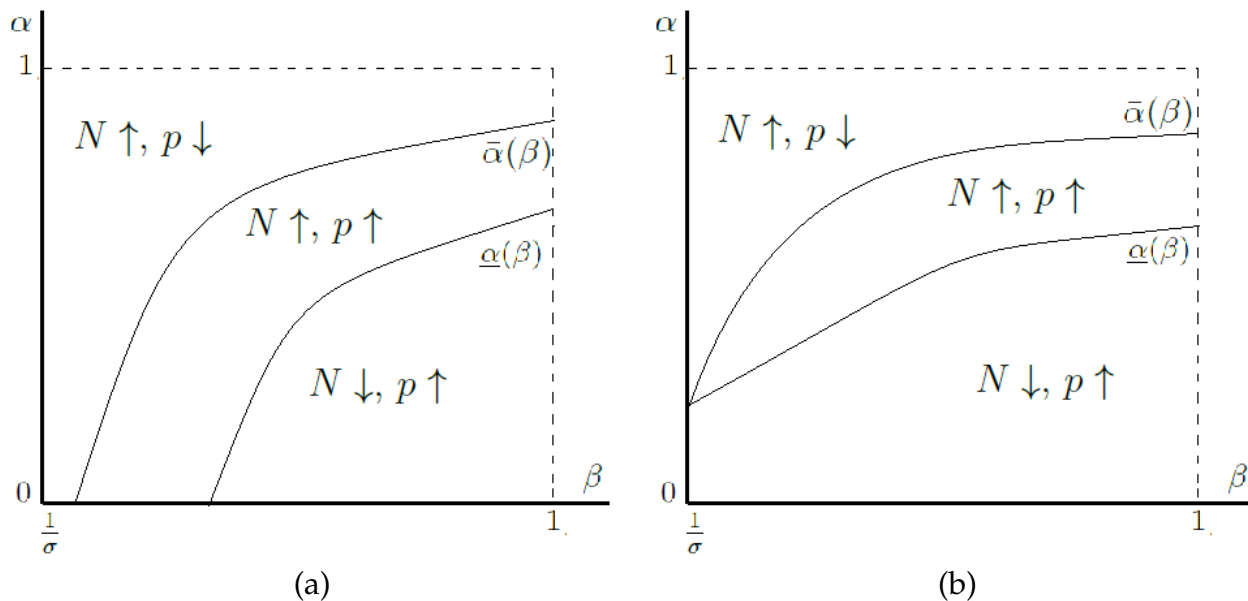
Figure 1: The pattern of market outcome: (a) \sigma > 1/\varepsilon ; (b) \sigma < 1/\varepsilon .
