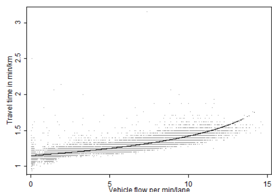
Figure 9 – Congested road
