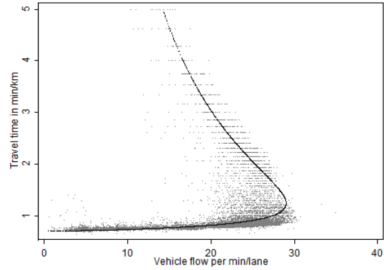
Figure 8 – Hypercongested road
