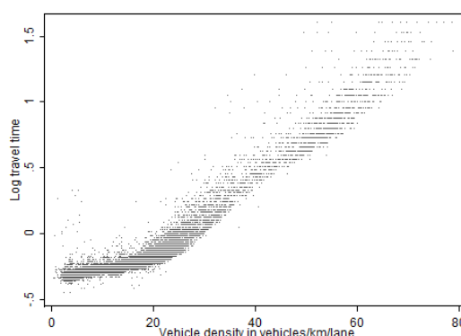
Figure 10 – Travel time-density
