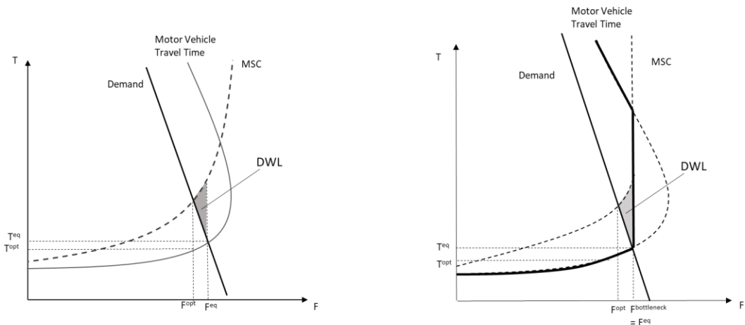
Figure 6 – Congested equilibria without (left panel) and with bottleneck (right panel)
