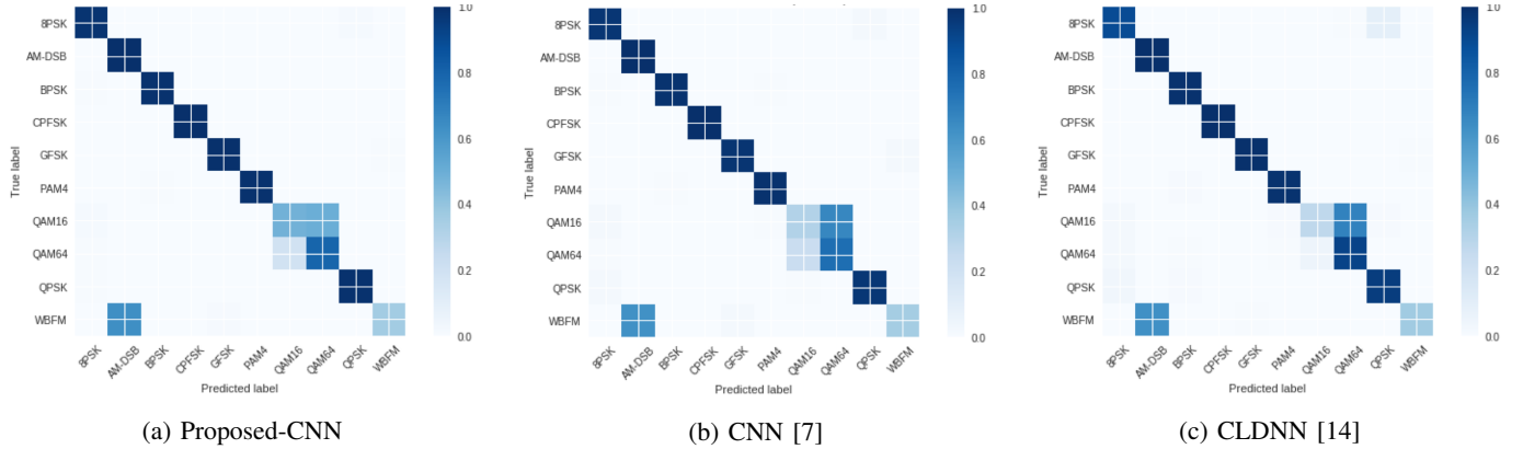
Fig. 4: Confusion Matrix at 18 dB SNRs
