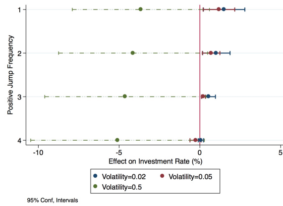
(c) Positive jump frequency ( \lambda^u )
