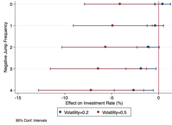
(b) Negative jump frequency ( \lambda^d )
