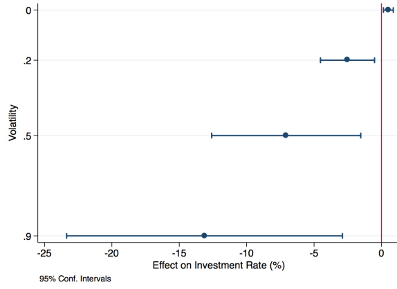
(a) Volatility ( \sigma )
