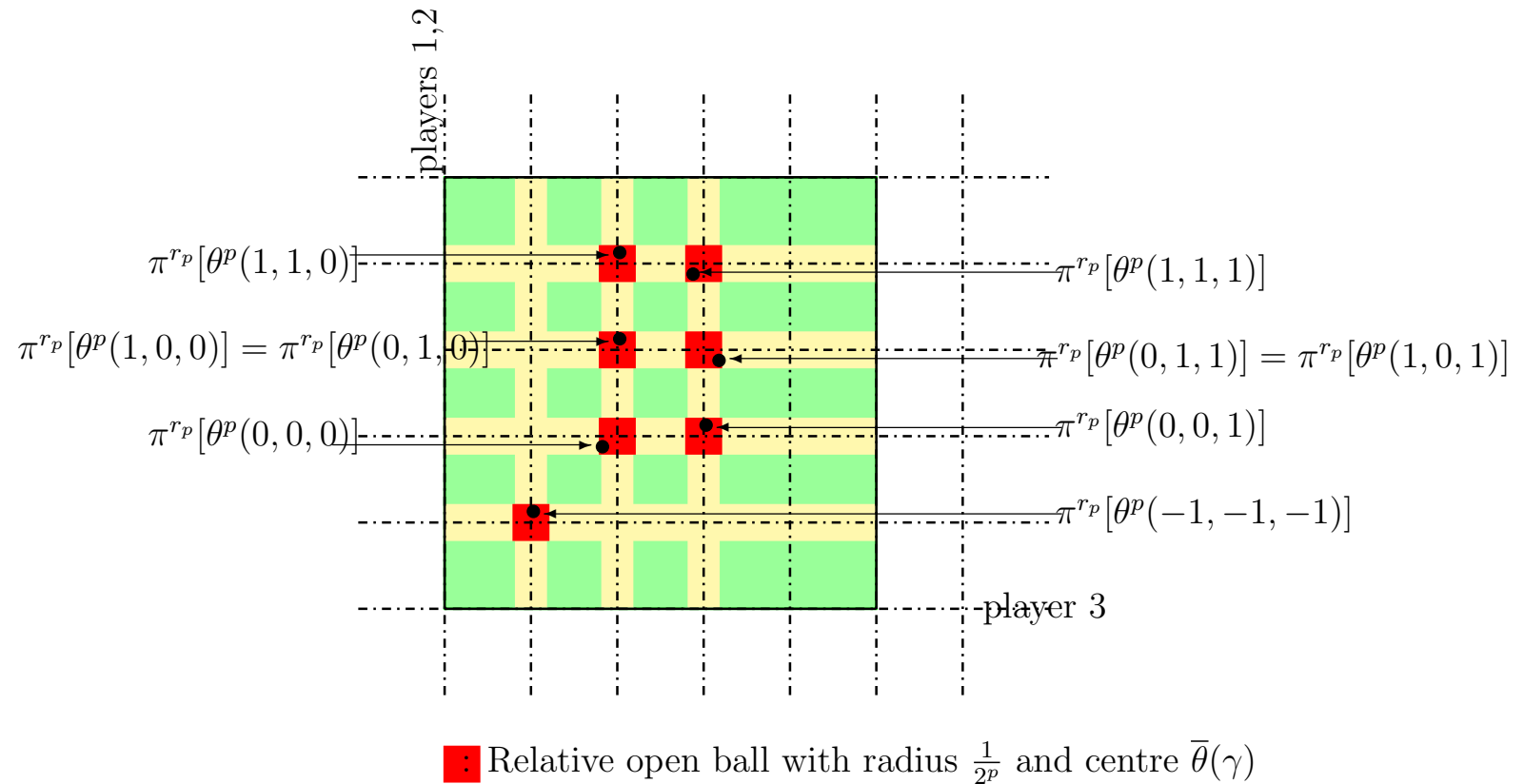
Figure 3: An example of relative position of the payoff vectors \pi^{r_p}[\theta^p(\gamma)] .
