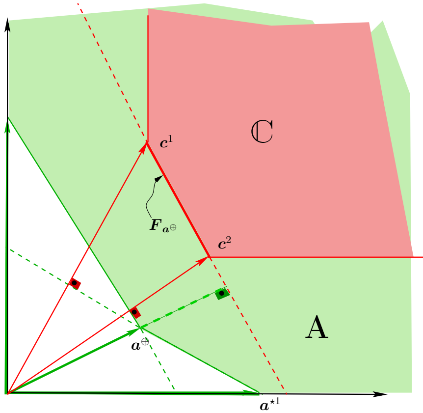
Figure 5.1: The shape of \mathbb{C} and \mathbf{A} – Two Dimensions
