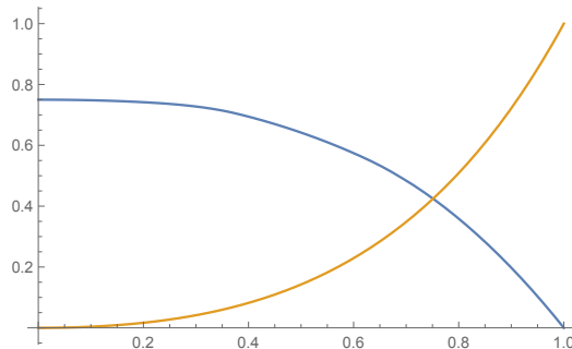
Figure 1: Exponential Neighborhood - Graphs of functions w_{t-2}(x) (decreasing) and \bar{r}_{T-2}(x) (increasing) for \alpha = -1 and \beta = 1 . The point of intersection is b_{T-2} .
