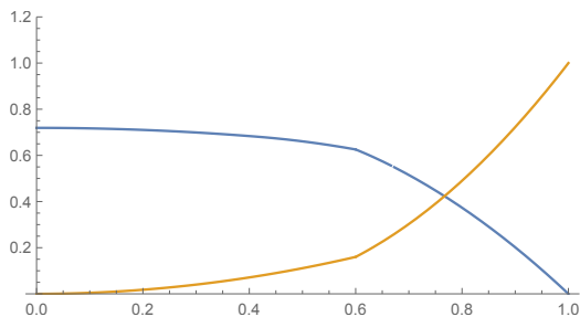
Figure 2: LCA n - Graphs of functions w_{t-2}(x) (decreasing) and \bar{r}_{T-2}(x) (increasing) for \lambda = 3/2 . The point of intersection is b_{T-2} .
