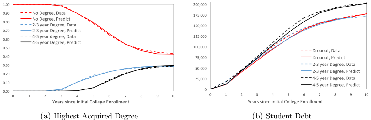
Figure 11: Model Fit
