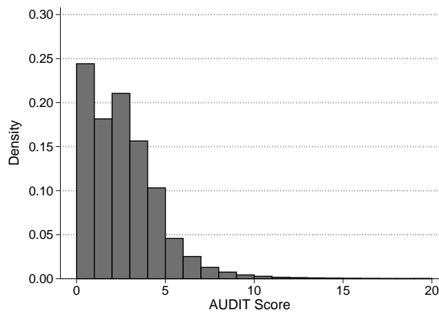
Figure 1 Distribution of AUDIT score 0-20
