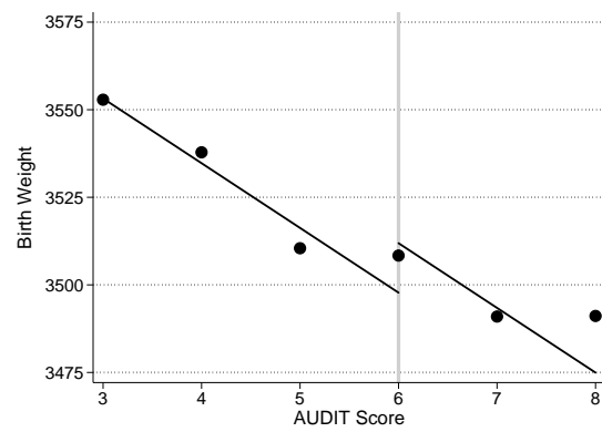
(b) 1st order joint polynomial, AUDIT 3-8
