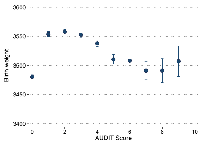
Figure 2: AUDIT score by birth weight
