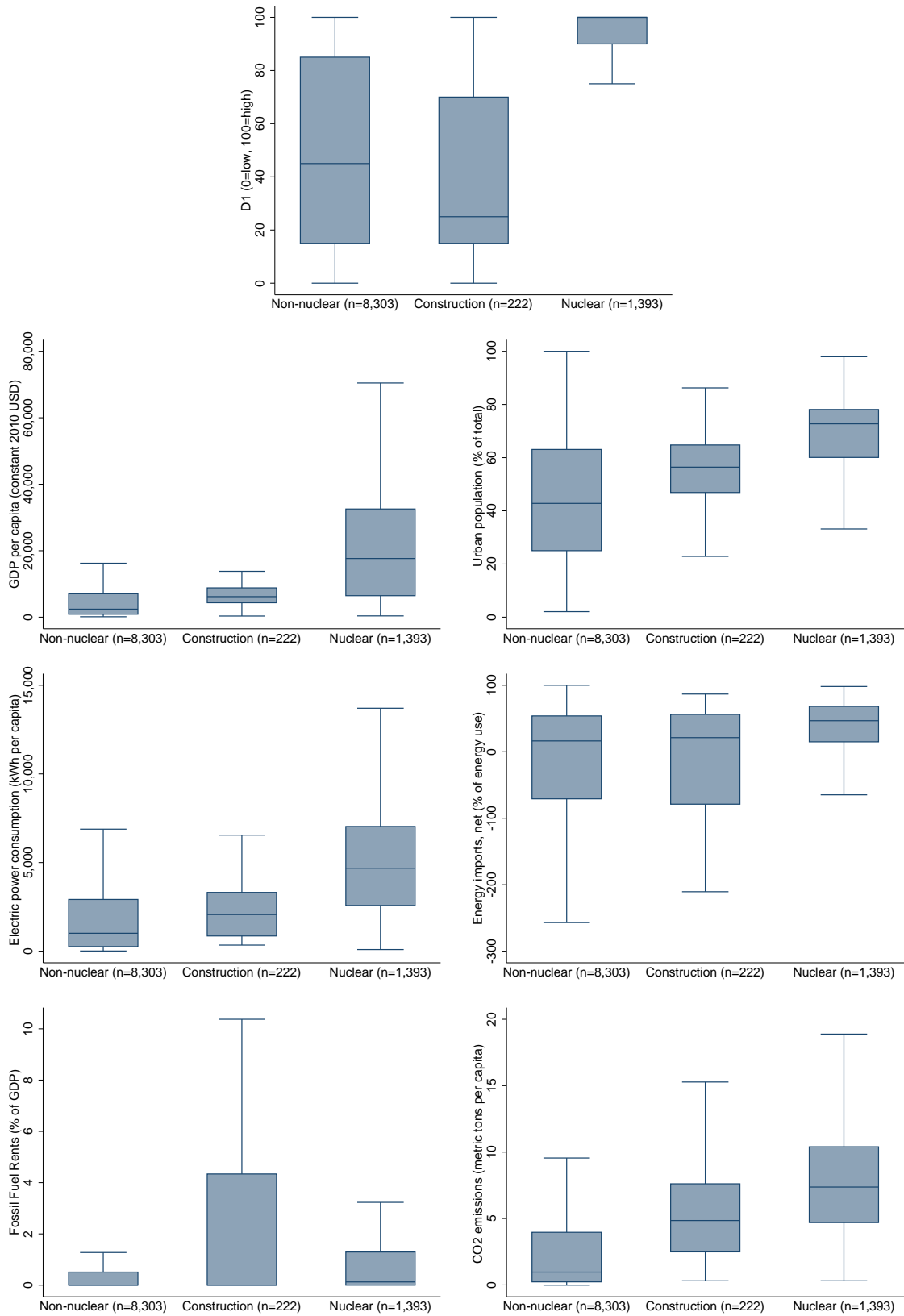
Figure 1: Boxplots for the three different nuclear energy statuses
