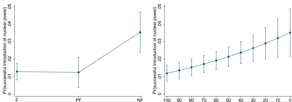
Figure 2: Adjusted predictions with 95% confidence interval for group membership of successful introduction of nuclear power by levels of democratic quality
