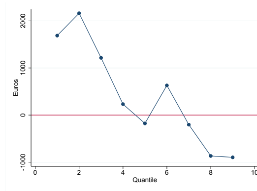
Figure 8: Quantile RDD estimates
