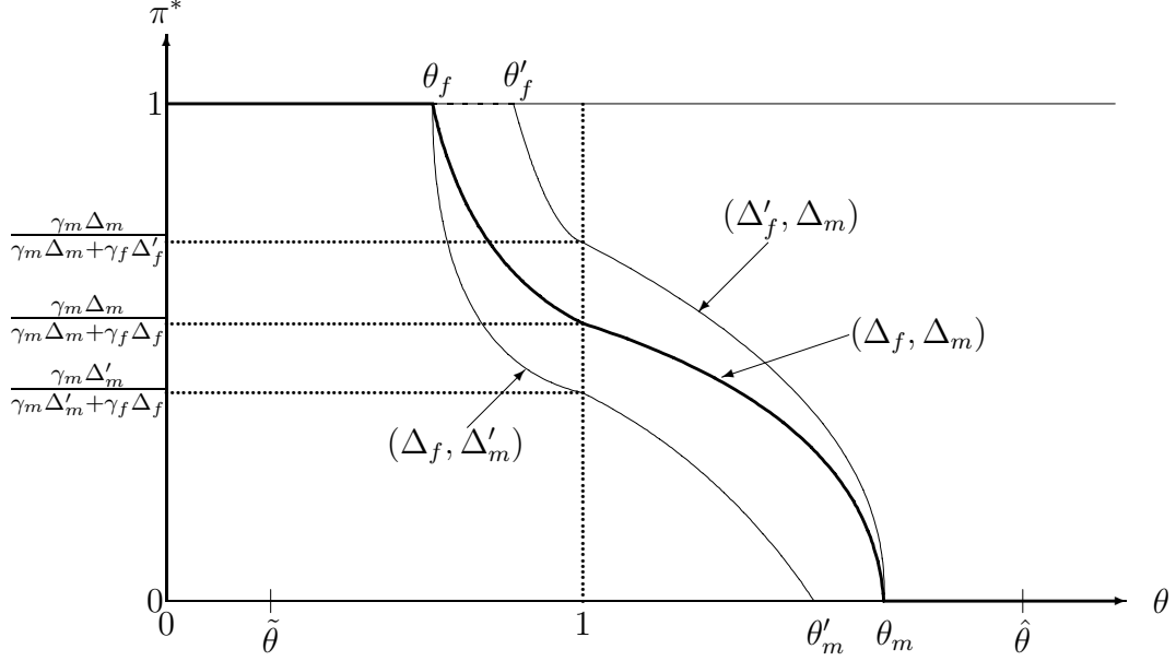
FIGURE 4. An illustration of Proposition 6 for three arbitrary and feasible pairs: (\Delta_f, \Delta_m) , (\Delta'_f, \Delta_m) and (\Delta_f, \Delta'_m) , where \Delta'_i < \Delta_i ( i = f, m ). Notice that for each i = f, m , \theta_i is the unique value of \theta such that \bar{\Delta}_i(\theta) = \Delta_i and \theta'_i is the unique value of \theta such that \bar{\Delta}_i(\theta) = \Delta'_i .
