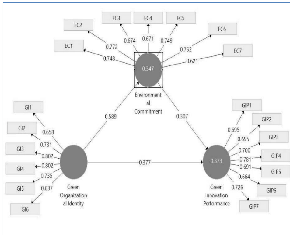
Figure 2: Measurement Model
