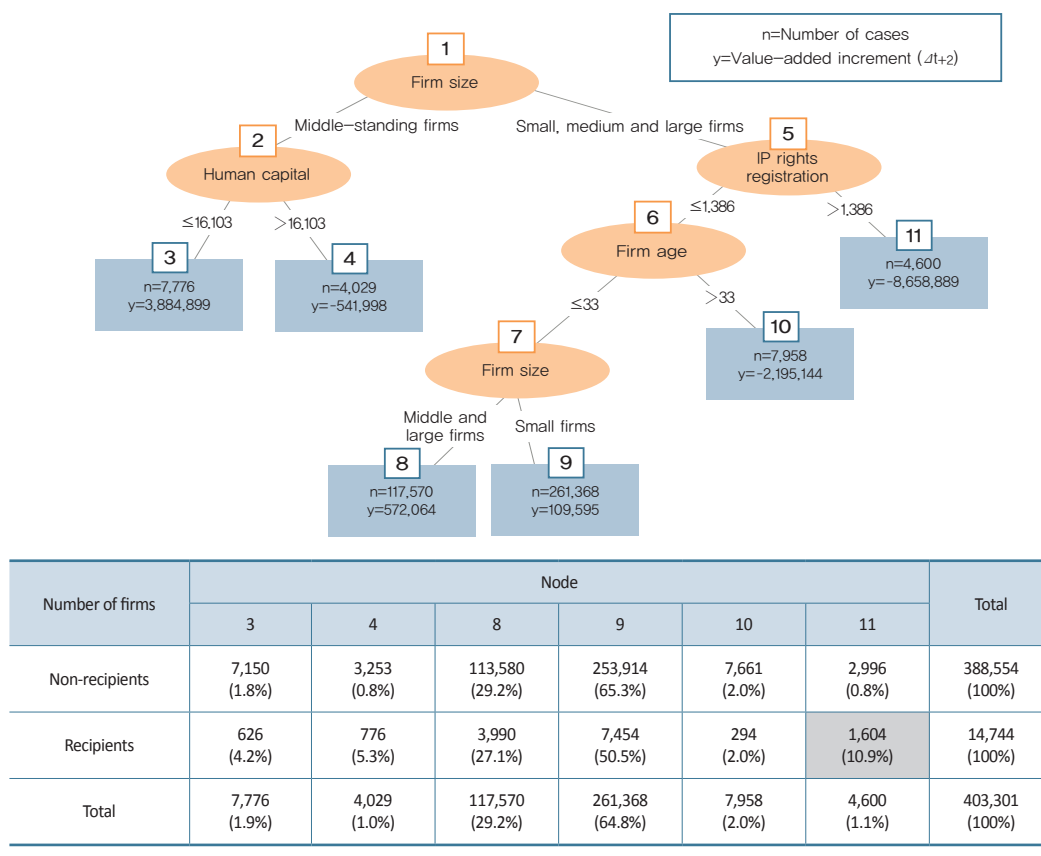
[Figure 1] Decision Tree Model Analysis for the Estimation of the Value Added Increment after Two Years (all firms)
