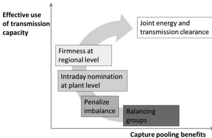
Figure 4: Balancing groups
