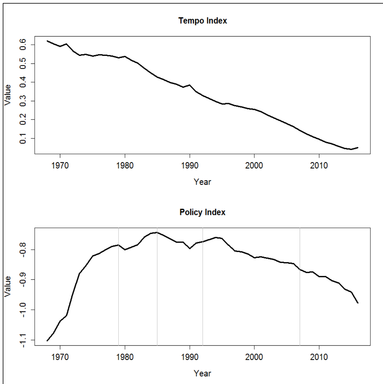
Fig. 5 Past courses of the first two principal components
