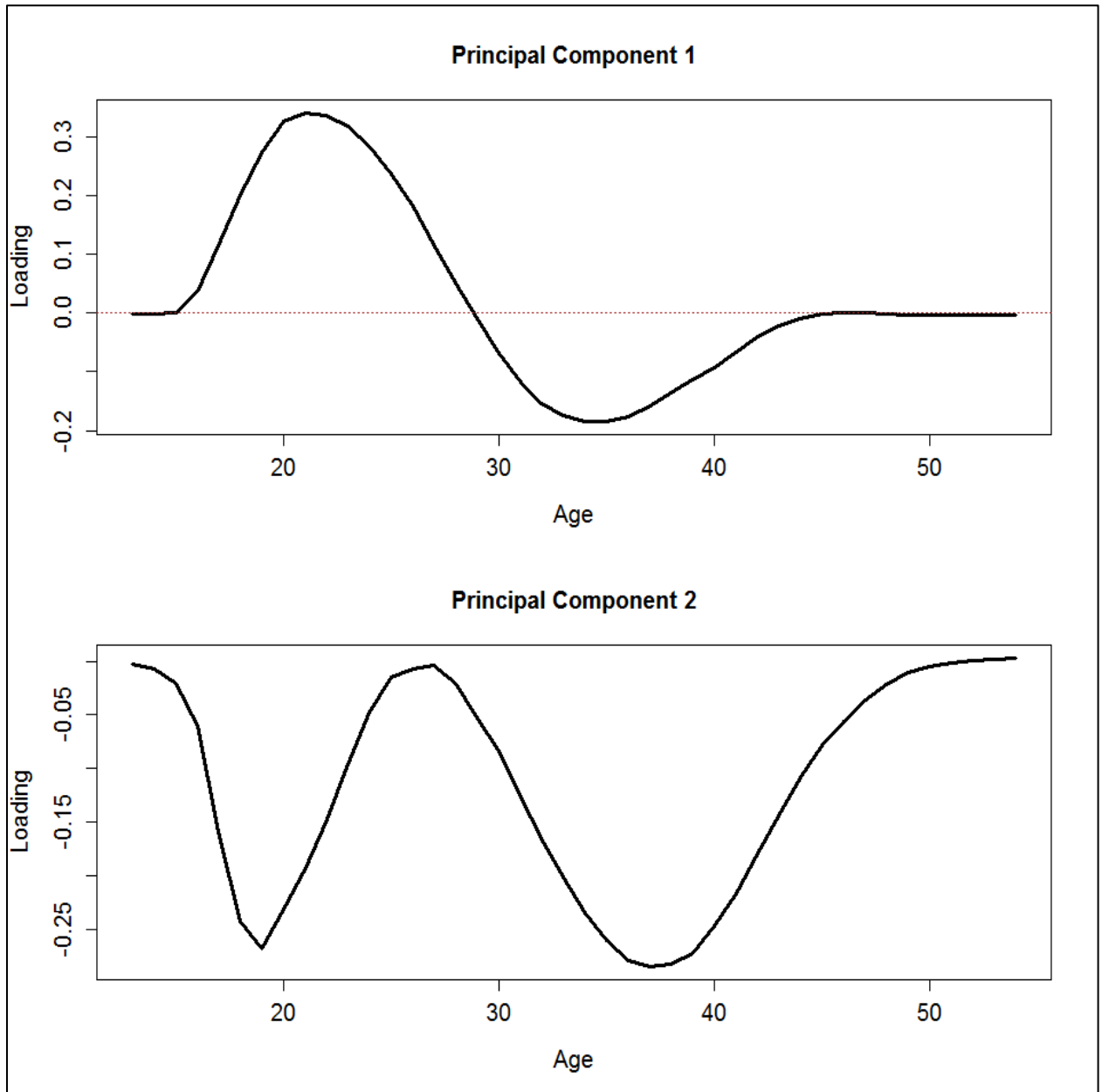
Fig. 4 Loadings of the first two principal components for the square roots of the age-specific fertility rates
