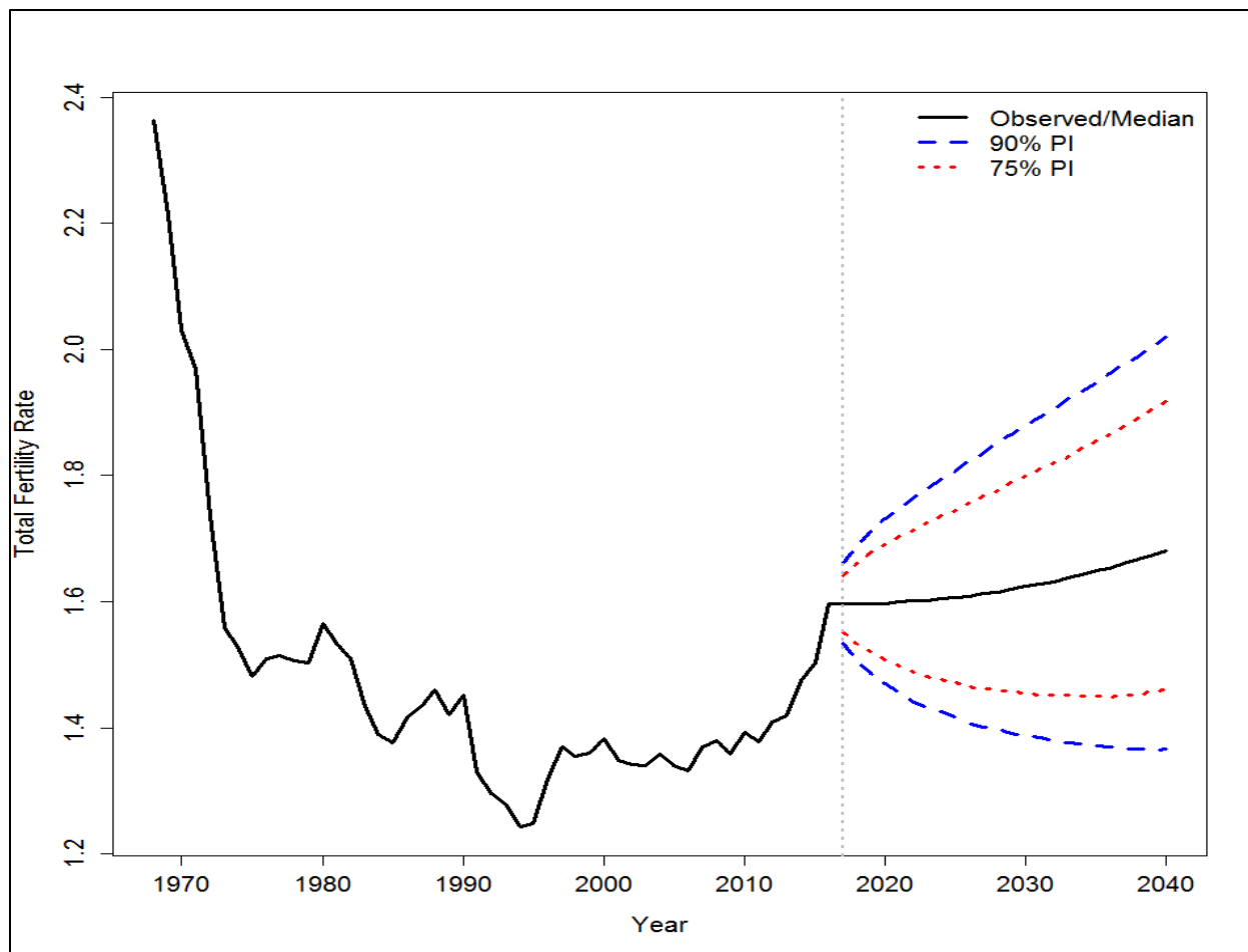
Fig. 8 Forecast of the total fertility rate
