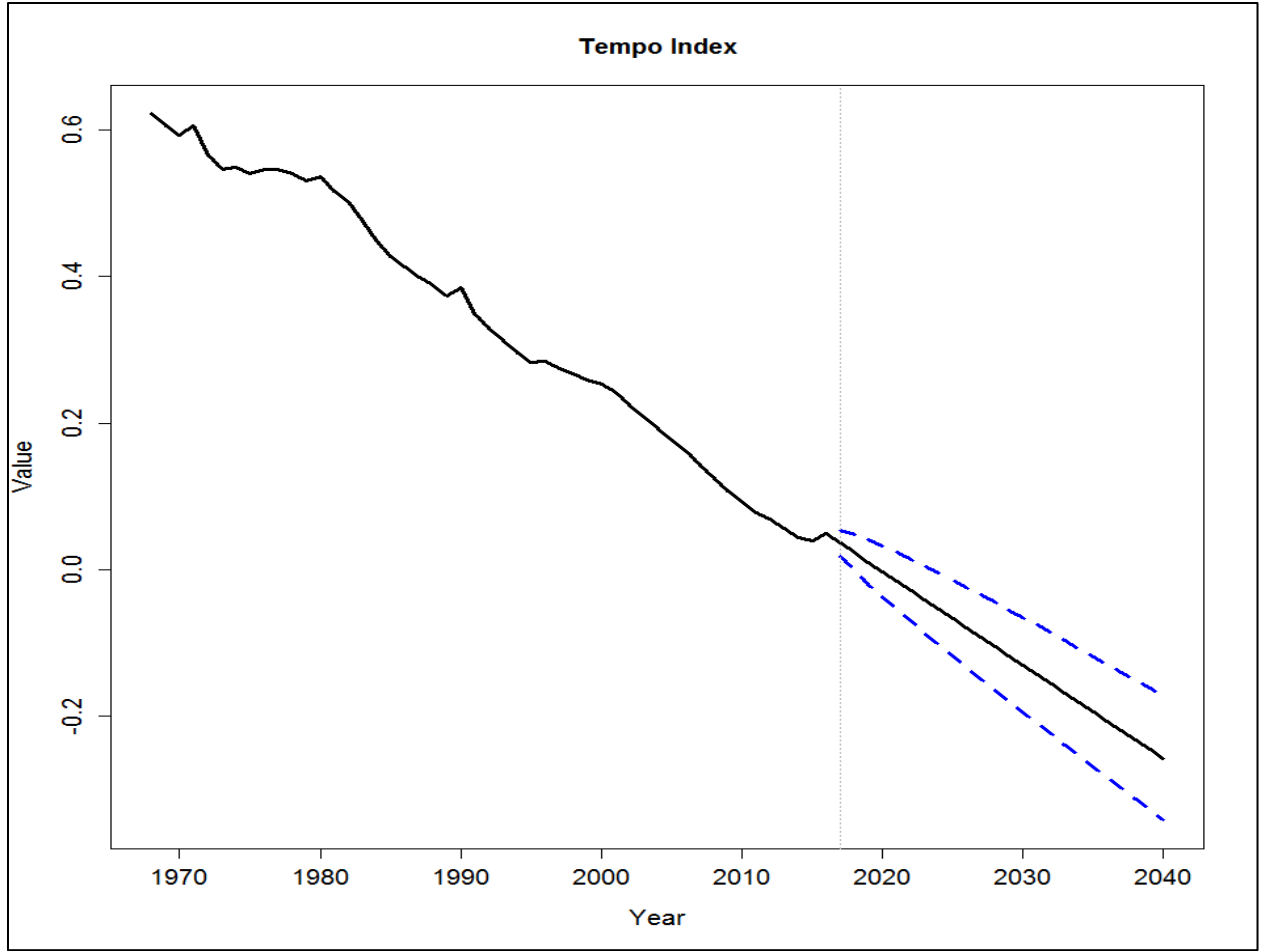
Fig. 6 Forecast of the Tempo Index
