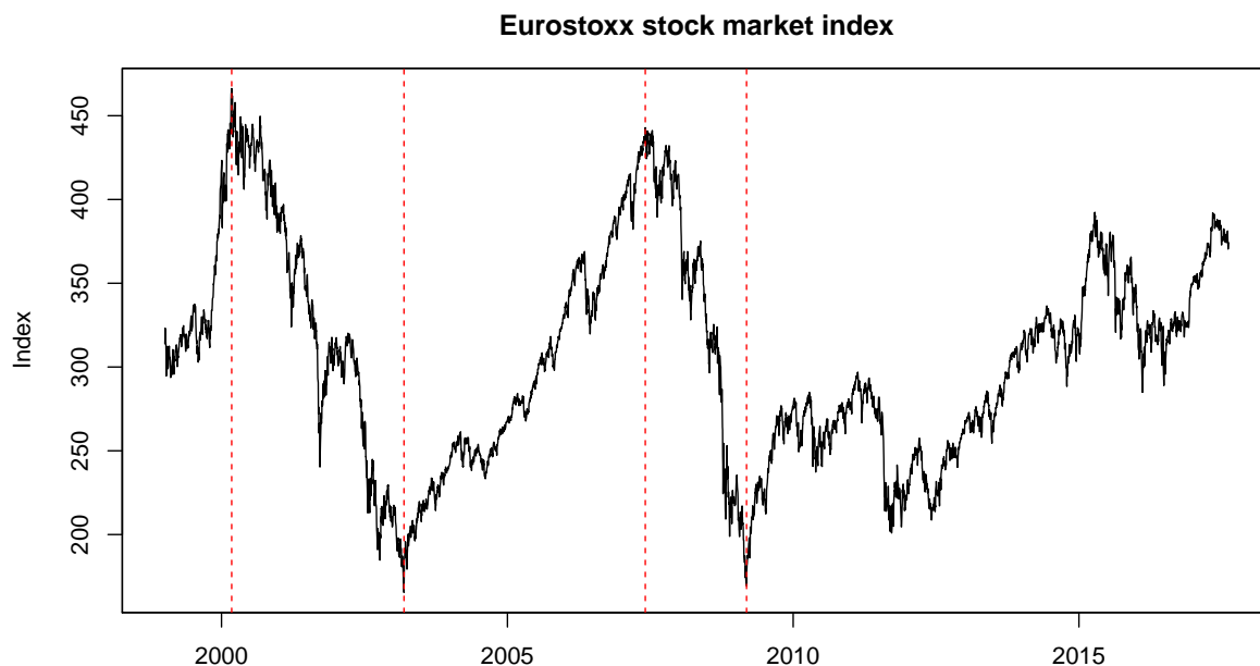
Figure 2: Development of the Eurostoxx stock market index and timing of bull and bear markets.
