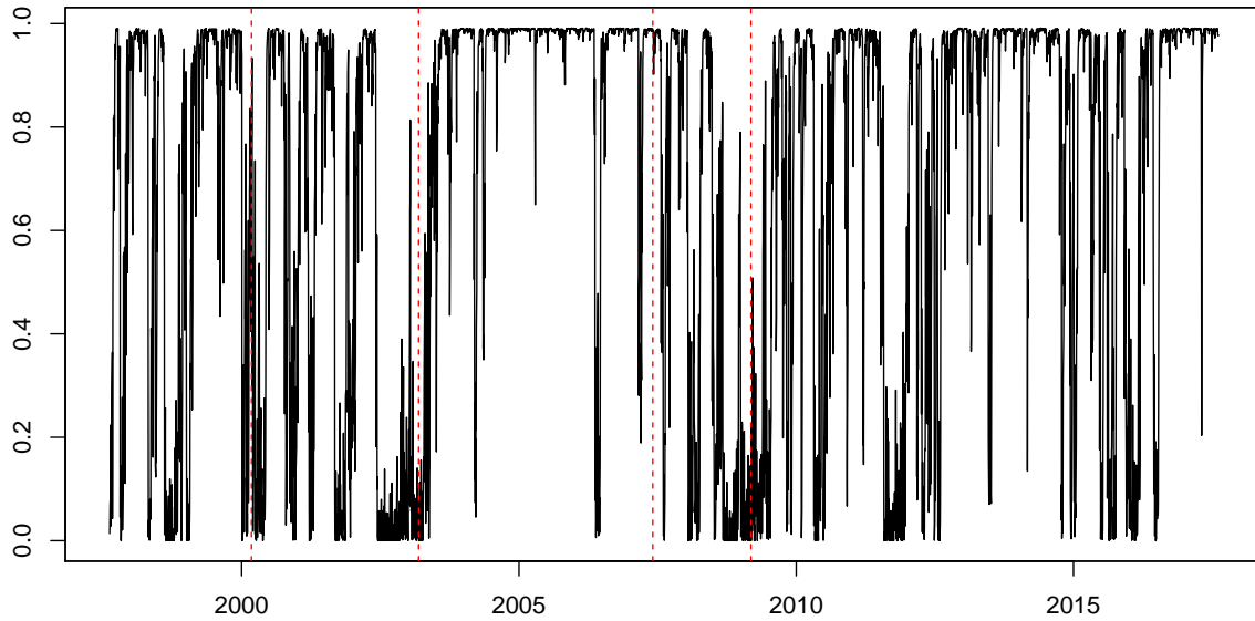
Bull-market probability of Markov-switching model
