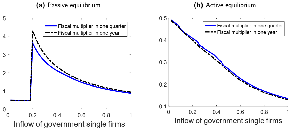
Figure 19: Fiscal multiplier
